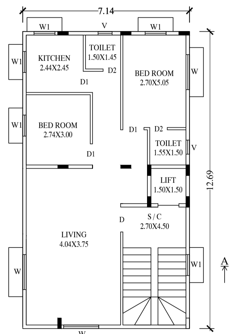
PRO. SECOND & THIRD FLOOR PLAN
