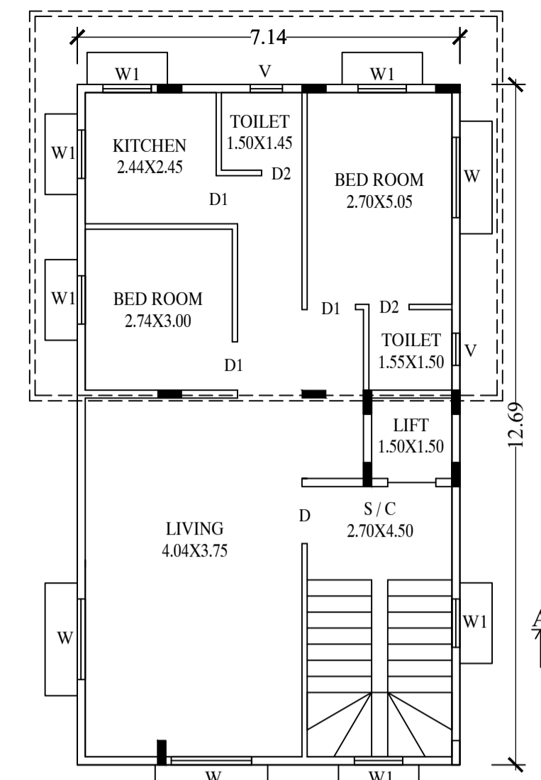
ADDITIONS TO EXISTING FIRST FLOOR
