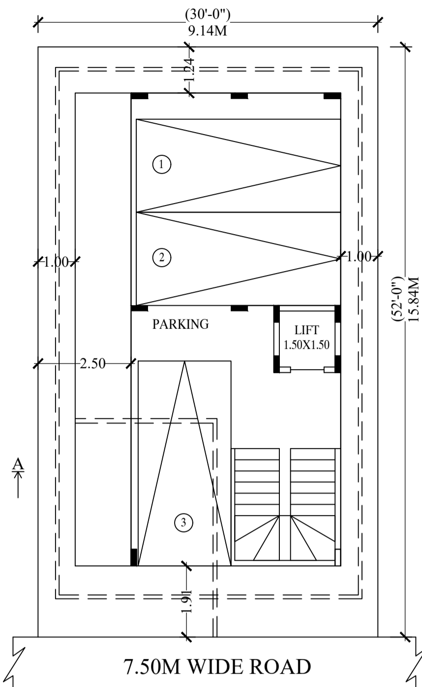
EX. GROUND FLOOR PLAN
